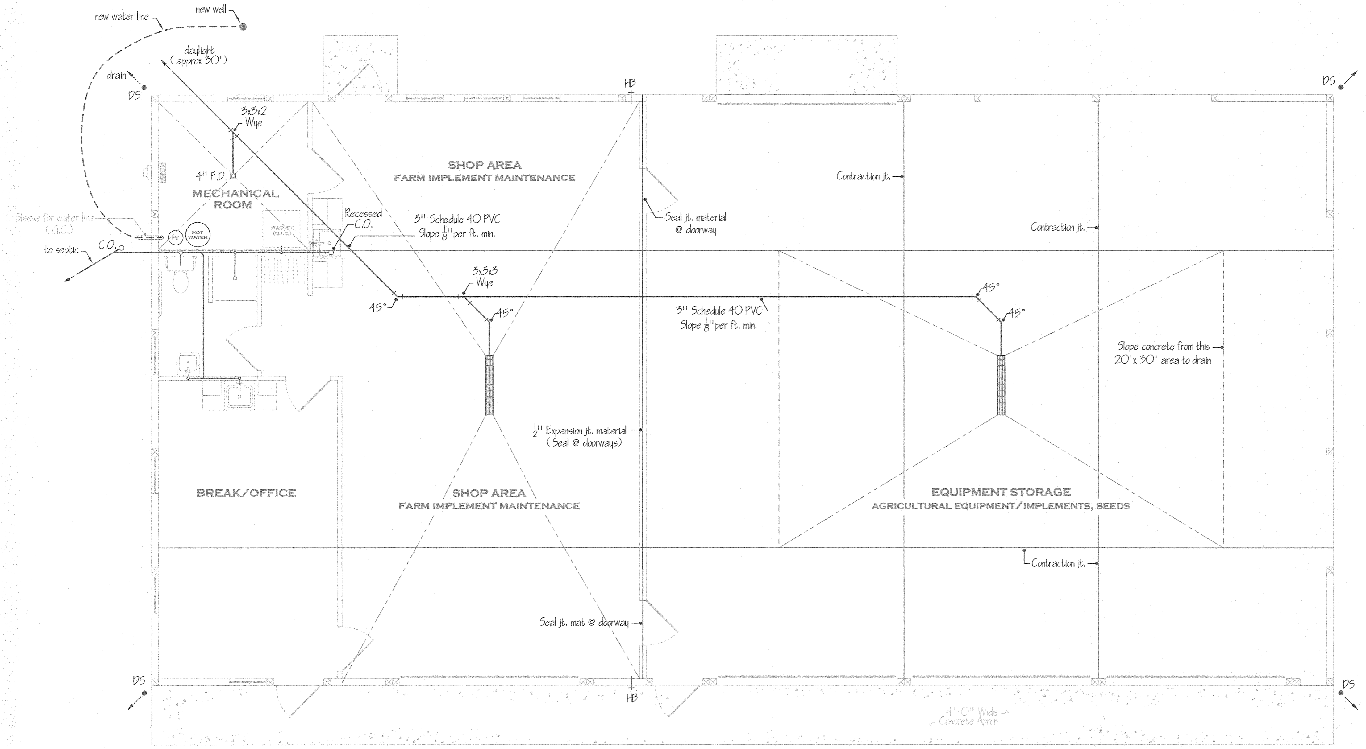
PLUMBING PLAN SCALE: 1/4" = 1'-0"
