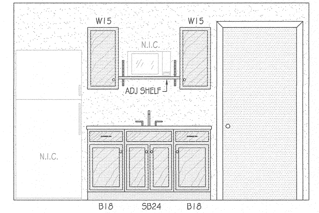
BREAK/OFFICE SCALE: 1/2" = 1'-0"
