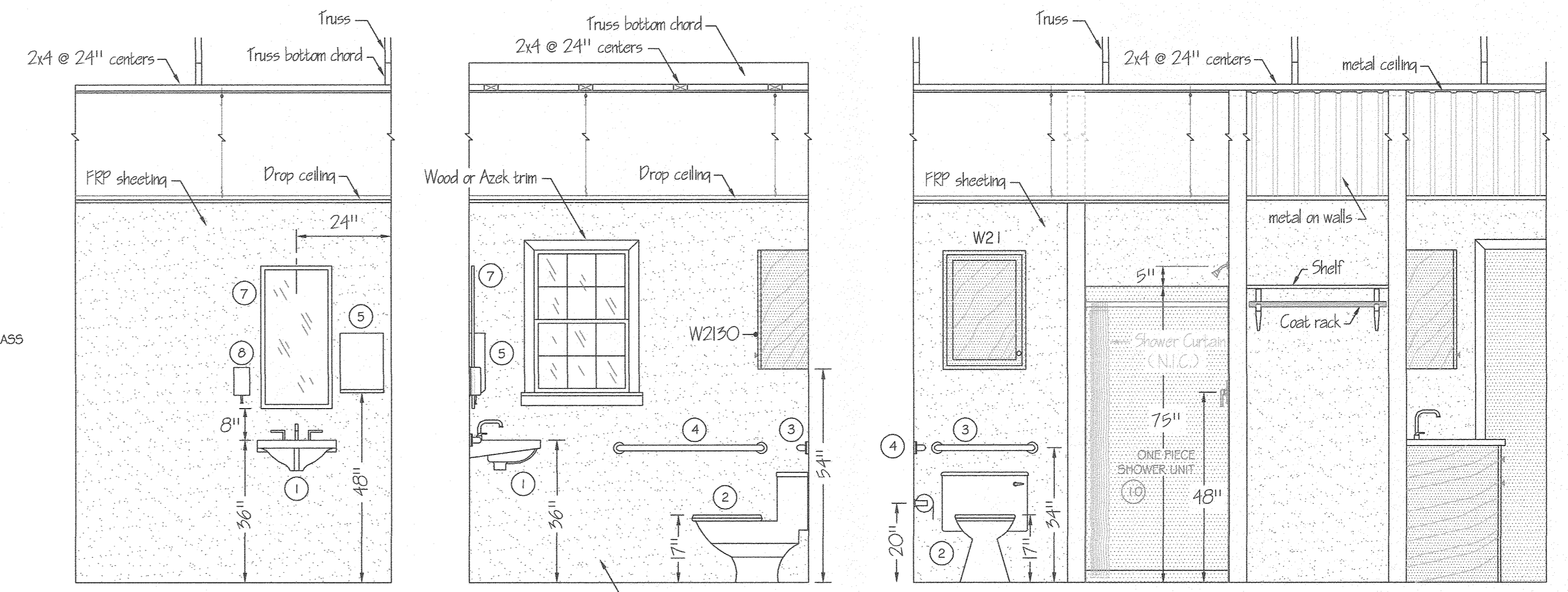
RESTROOM ELEVATIONS SCALE: 1/2" = 1'-0"
